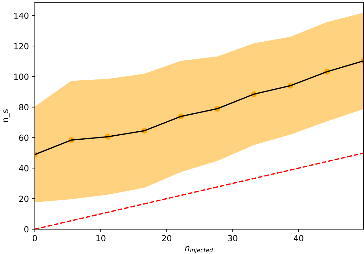
Bias ( n_s )
