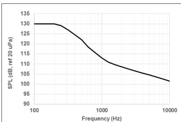
Figure 6: Payload acoustic environment (1/3 octave)
