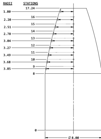
Figure 4: Starship payload volume (dimensions in m)
