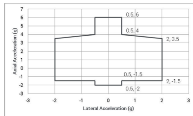
Figure 5: Payload maximum design load factors
