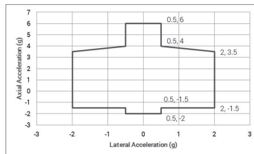
Figure 5: Payload maximum design load factors
