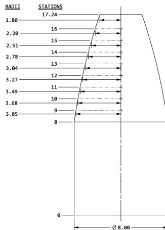
Figure 4: Starship payload volume (dimensions in m)
