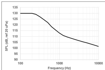
Figure 6: Payload acoustic environment (1/3 octave)
