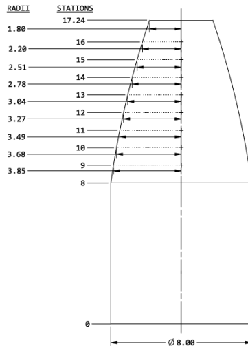
Figure 4: Starship payload volume (dimensions in m)
