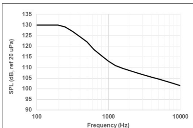
Figure 6: Payload acoustic environment (1/3 octave)
