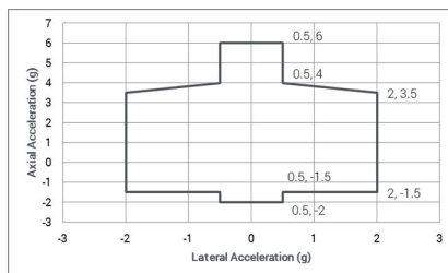
Figure 5: Payload maximum design load factors
