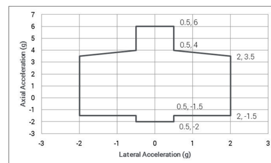
Figure 5: Payload maximum design load factors
