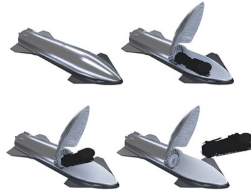
Figure 3: Starship payload deployment sequence
