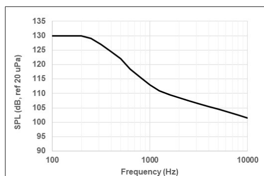
Figure 6: Payload acoustic environment (1/3 octave)
