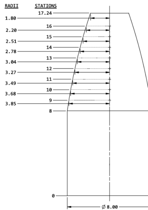
Figure 4: Starship payload volume (dimensions in m)
