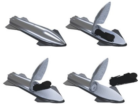
Figure 3: Starship payload deployment sequence
