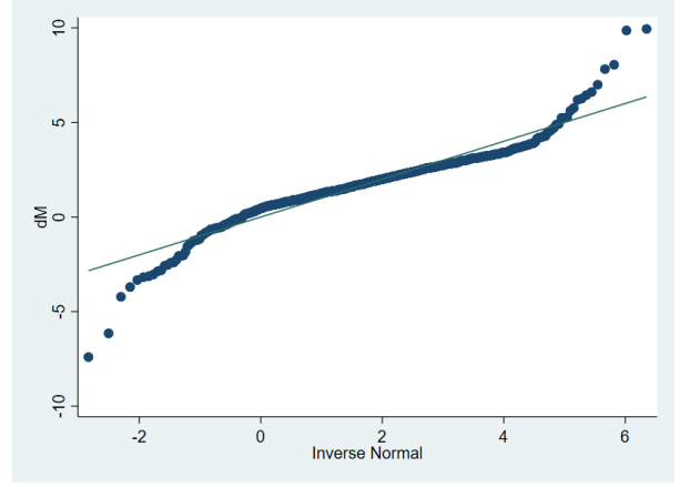
(b) Q-Q wrt normal distribution
