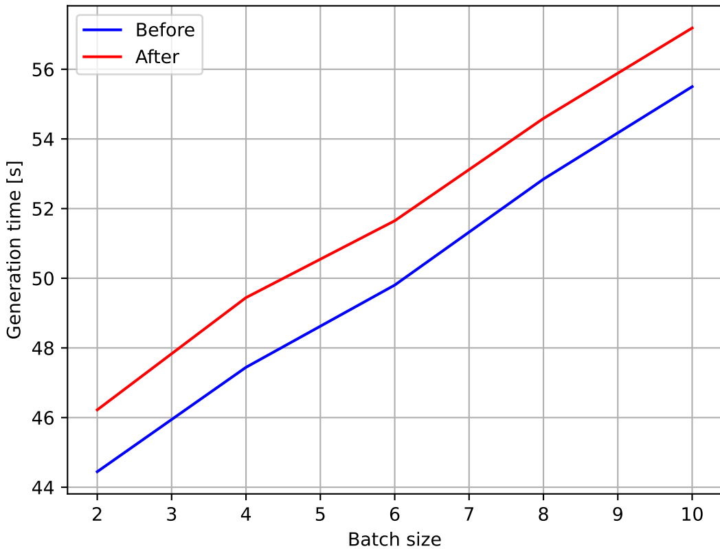
Meta-Llama-3-8B Input size 300, New tokens 2000
