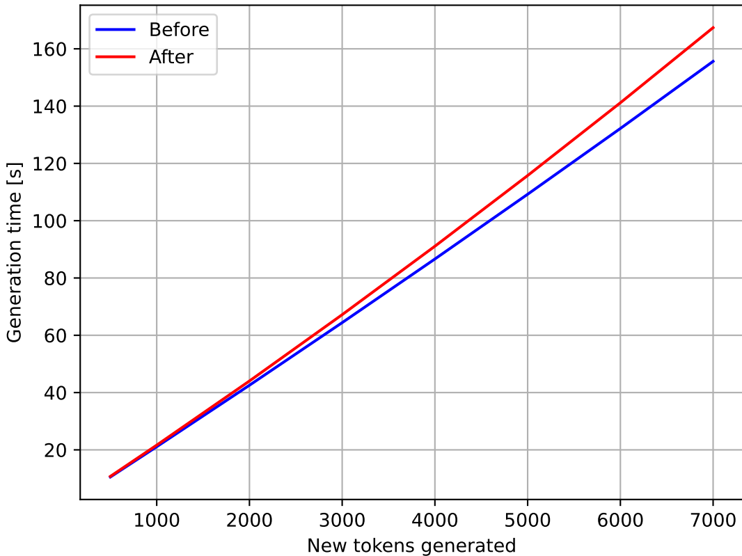
Meta-Llama-3-8B Input size 300, Batch size 1
